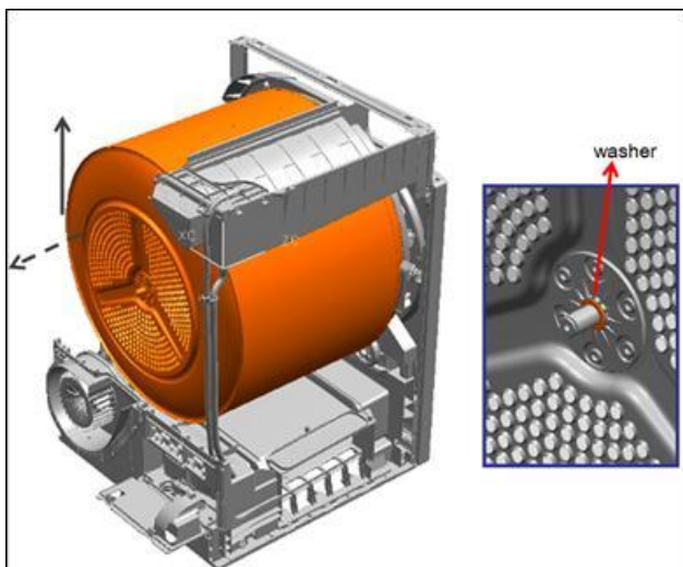
Figure 11.15. Drum Disassembly
