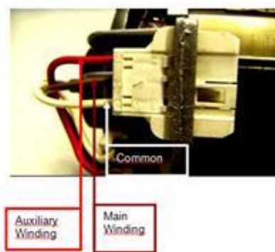
Figure 4.6. Asynchronous Motor
