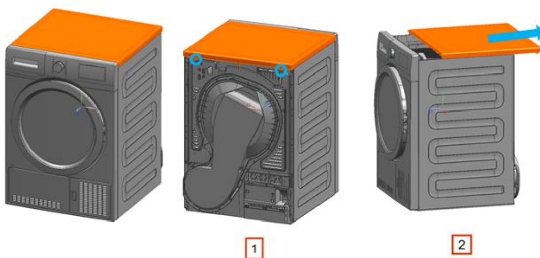
Figure 11.2. Disassembling the top plate
