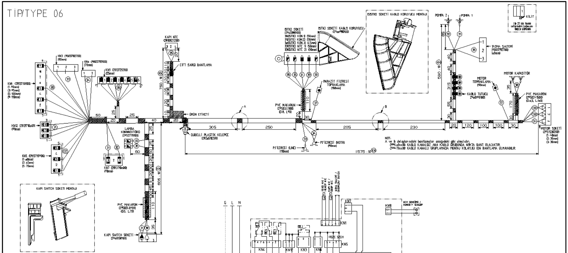
Figure 11-3: Cable Schematics (2994600600) – Beko 2013 Good+ CNDU Models Opaque Door 60 cm
